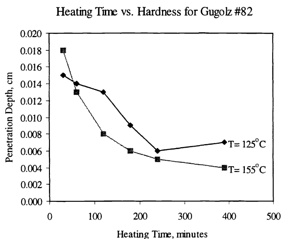
Figure 3 The effect of heating (melting) time on pitch hardness
