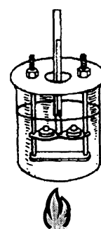
Figure 4 Softening point apparatus
