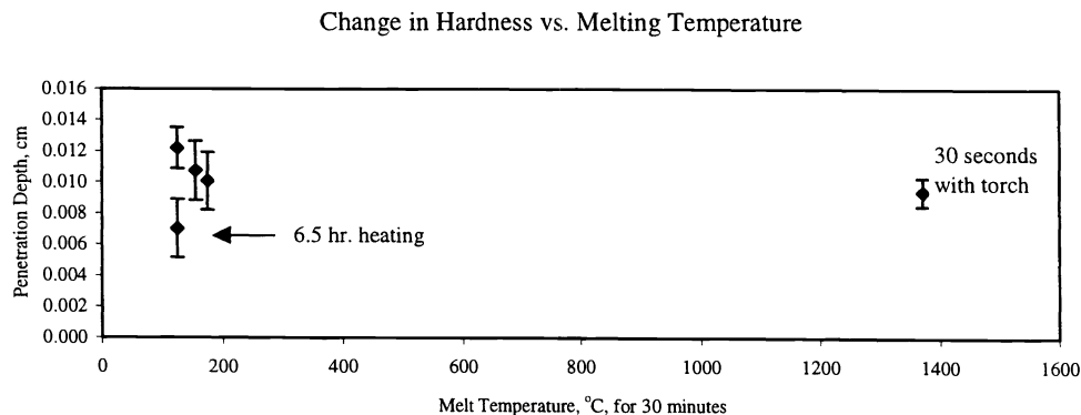
Figure 2 The effect of pitch melt temperature on hardness
